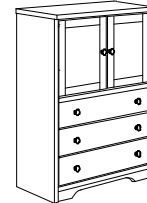
774 2 Door/3 Drawer Chest 31 1/2" W x 16" D x 51 1/2" H
